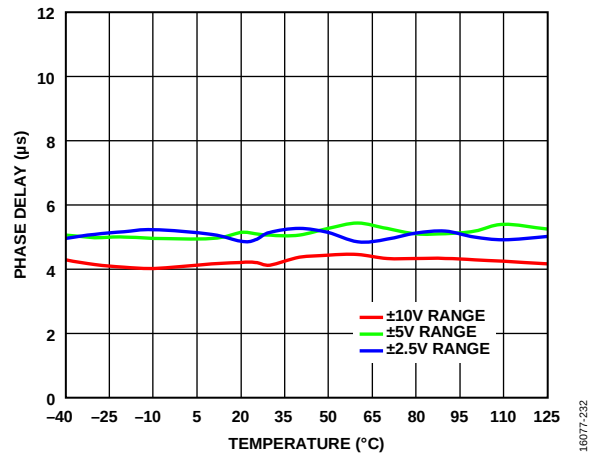
Figure 32. Phase Delay vs. Temperature
